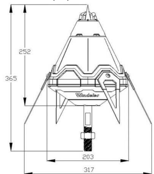
Dimensions (mm)
